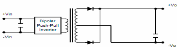
Single Output
