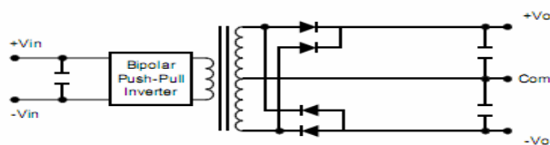
Dual Output
